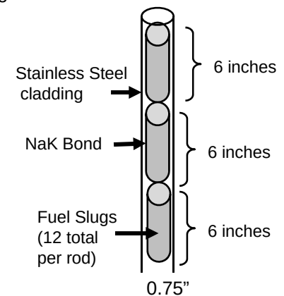
Fuel Rod
